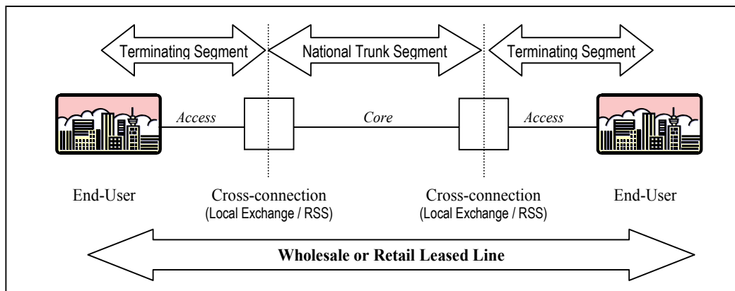
Figure 1 - Segments of an end-to-end leased line
